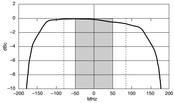
Figure 2. Measured Modulation Bandwidth at 2.4 GHz Carrier Frequency
